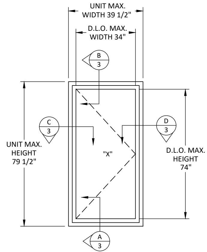
TYPICAL ELEVATION
