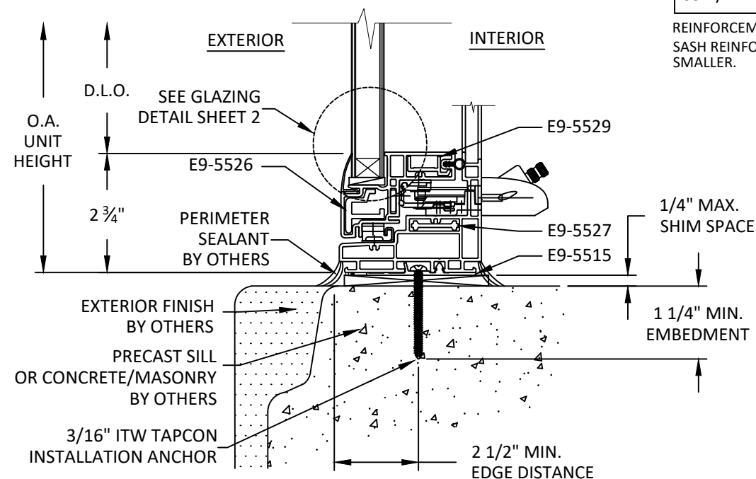
A 3 VERTICAL SECTION SILL - CONCRETE/MASONRY THROUGH CLIP
