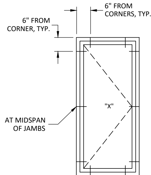
ANCHOR LAYOUT WINDOW WIDTH ≤ 35.5"
