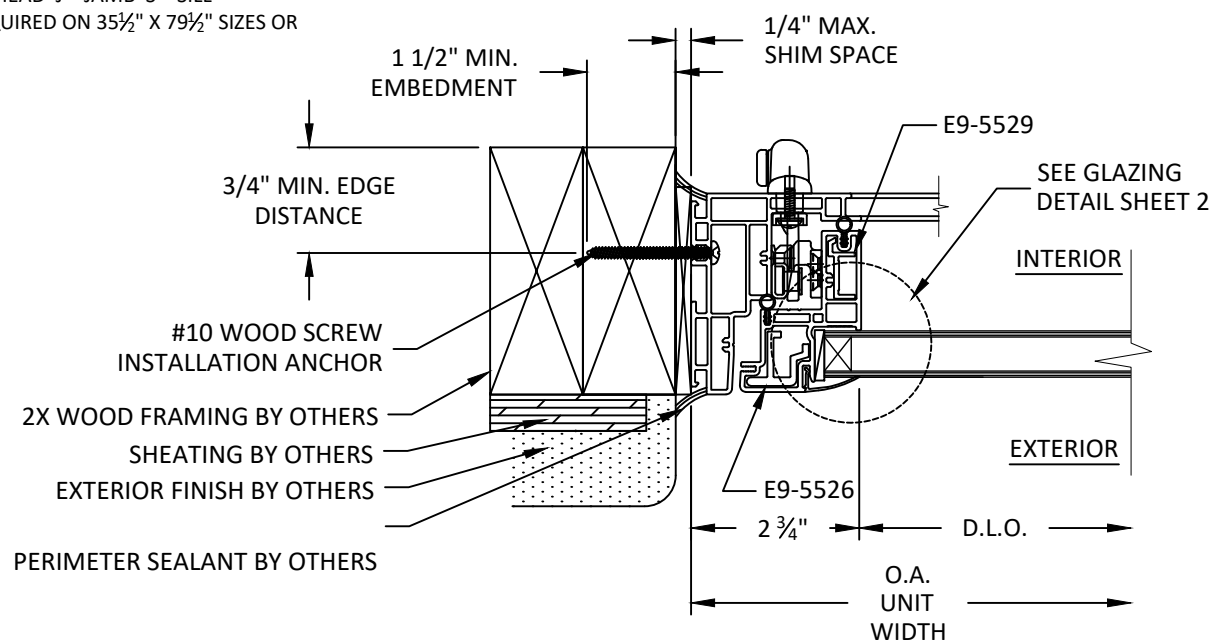
C 3 HORIZONTAL SECTION JAMB - 2X WOOD FRAMING THROUGH FRAME
