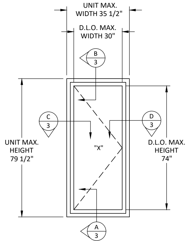
TYPICAL ELEVATION
