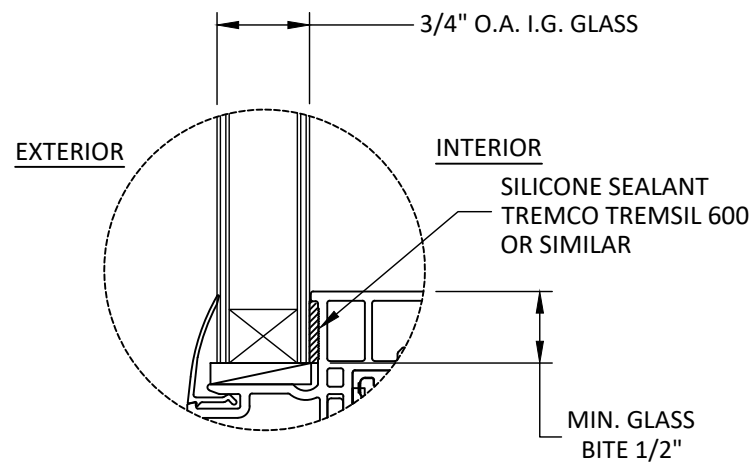
GLAZING DETAIL
