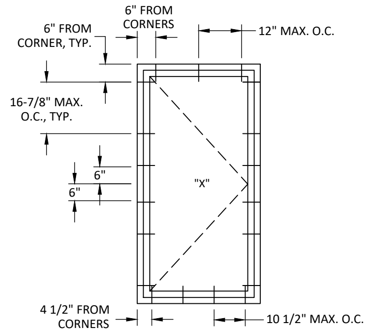
ANCHOR LAYOUT WINDOW WIDTH > 35.5"
