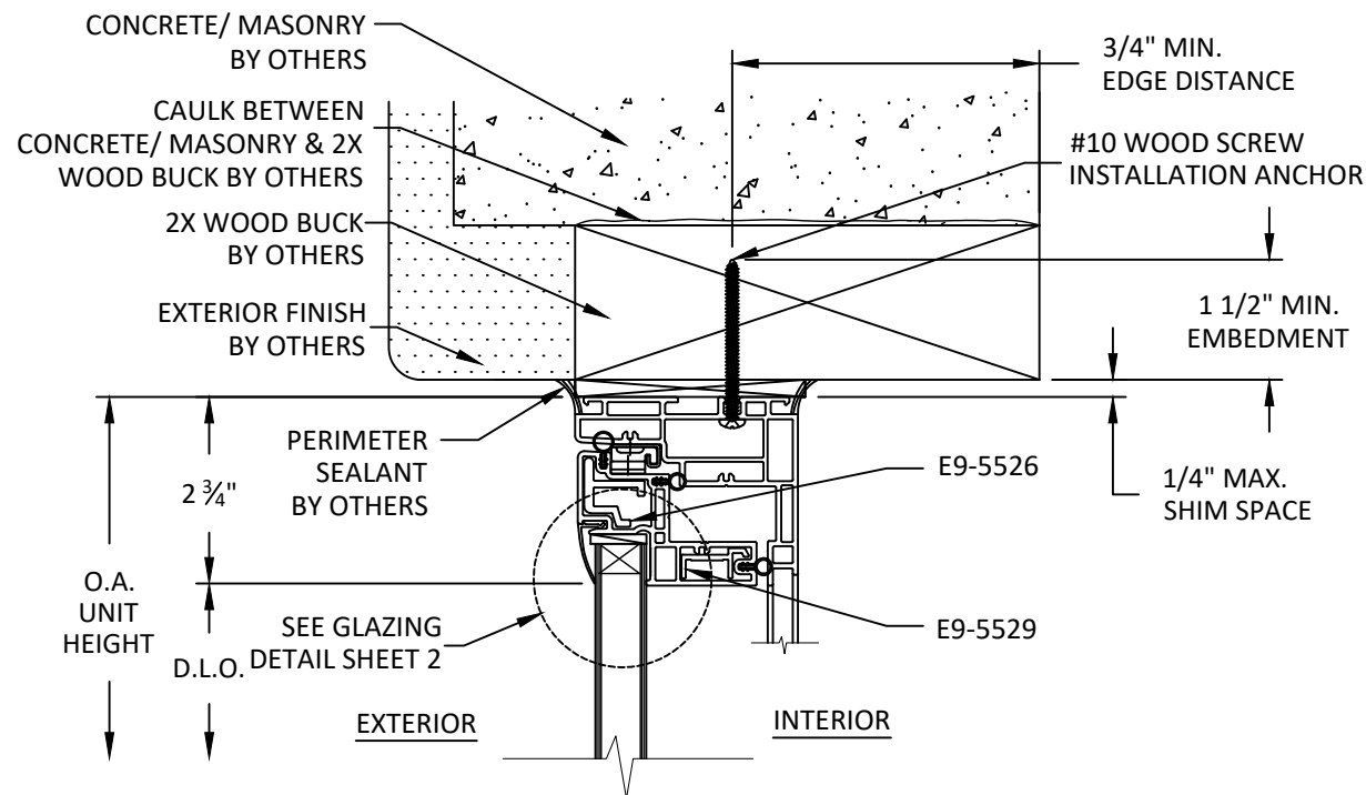
B 3 VERTICAL SECTION HEAD - 2X WOOD BUCK THROUGH FRAME
